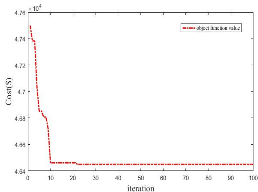
Fig. 11. Convergence of the PSO-GA.
