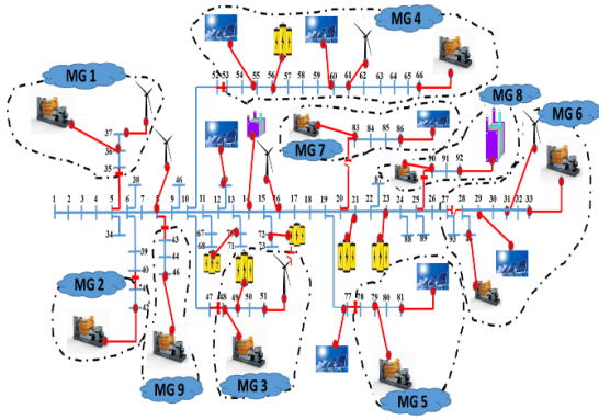
Fig. 8. Optimal site of DER, ESS and DGs in MGs and the State of MGs
