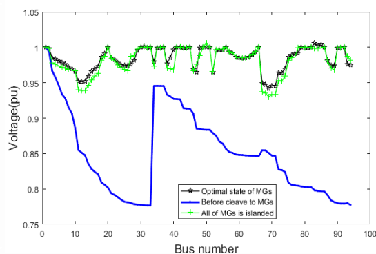
Fig. 10. Voltage profile of system in the three scenarios
