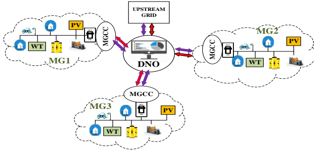
Fig. 2. Networked-MGs and two-way exchange of energy and data
