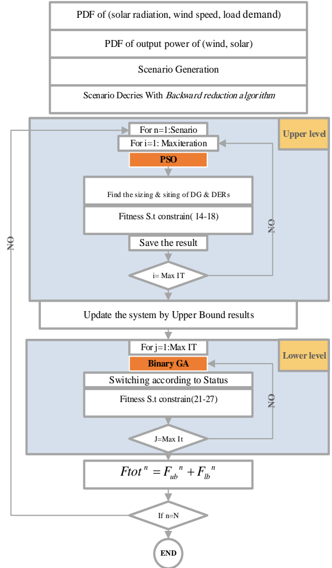
Fig. 6. Flowchart of the proposed bi-level approach to solving the problem.
