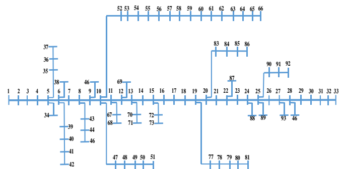
Fig. 1. The 94-bus distribution network of Portugal [13]
